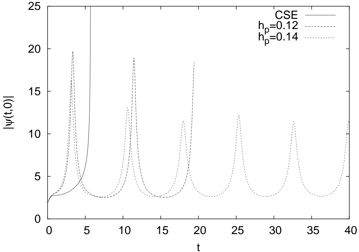
FIG. 1: h = 1.95 , w_p = 0.5 : oscillations in place of collapse.
