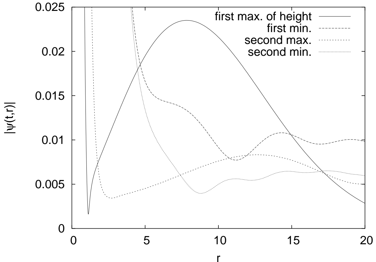
FIG. 4: h = 1.95, h_p = 0.14, w_p = 0.5 |\psi(t, \cdot)| profiles: inner-outer separation.
