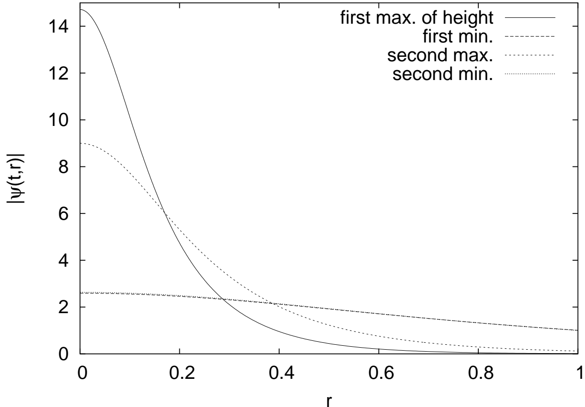
FIG. 3: h = 1.95, h_p = 0.14, w_p = 0.5 |\psi(t, \cdot)| profiles showing oscillations in Townes soliton form.
