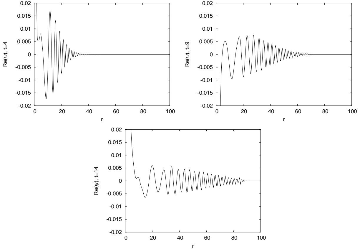
FIG. 6: h = 1.95, h_p = 0.14, w_p = 0.5 \Re(\psi) vs. r at t = 4, 9, 14 , showing radiation.
