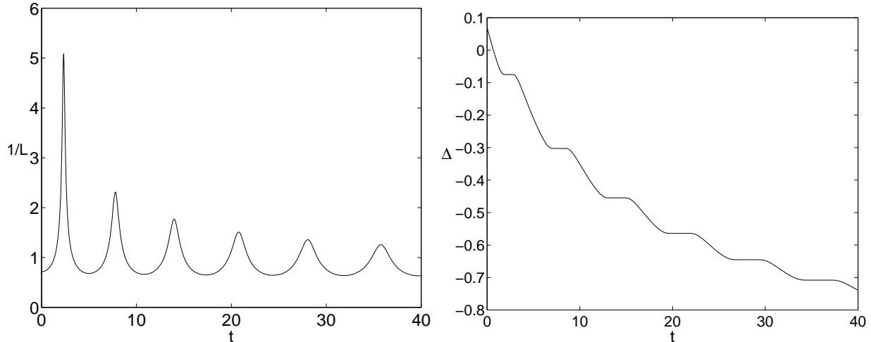
FIG. 2: Collective coordinates approximations with the sech approximation of the Townes soliton, L(0) = 1.4 , L'(0) = 0 , \Delta(0) = 0.07 , w_p = 0.5 , h_p = 5 .
