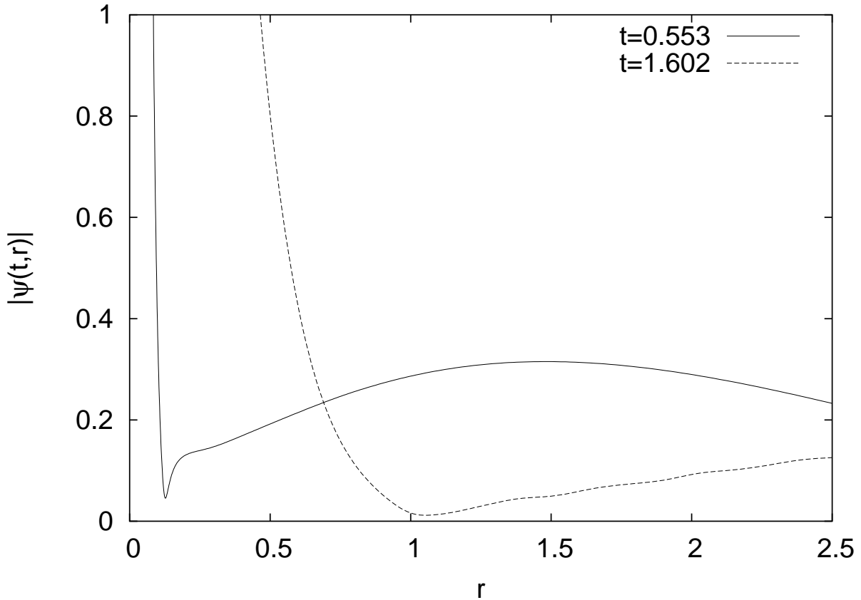
FIG. 5: h = 2.1, h_p = 3.48, w_p = 0.3 , |\psi(t, \cdot)| with extreme splitting of beam power; near maximum ( |\psi(0.553, 0)| = 115 and minimum ( |\psi(1.602, 0)| = 11 of focusing oscillations.
